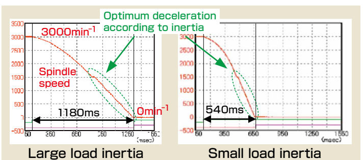
Optimum orientation (example)
